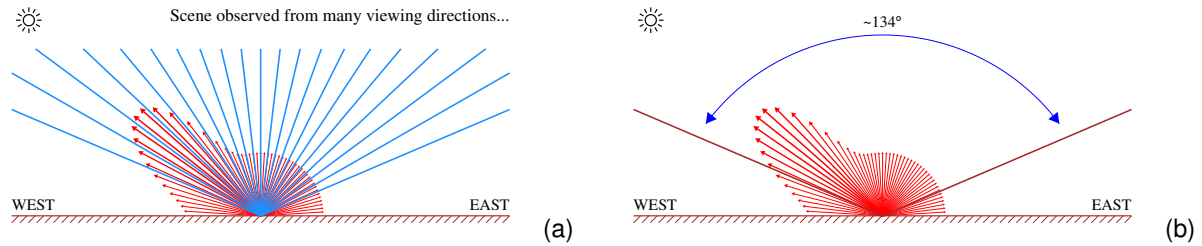
Figure 11: Left: During one month of observations, a certain location is observed many times by TROPOMI for many different viewing geometries (angles). At the equator, each location is observed roughly 30 times per month. Right: The range in viewing angles covered this way is approximately 134 degrees.
