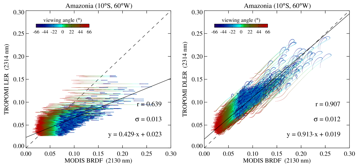
Figure 22: Left: TROPOMI surface LER versus MODIS surface BRDF for a region in the Amazonian rainforest. Right: The same plot, but now with TROPOMI surface DLER on the vertical axis.
